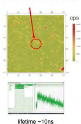
nanodiamond with NV centre
